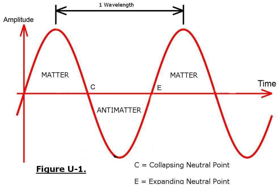
Figure U-1. Cycle of our blinking universe.
